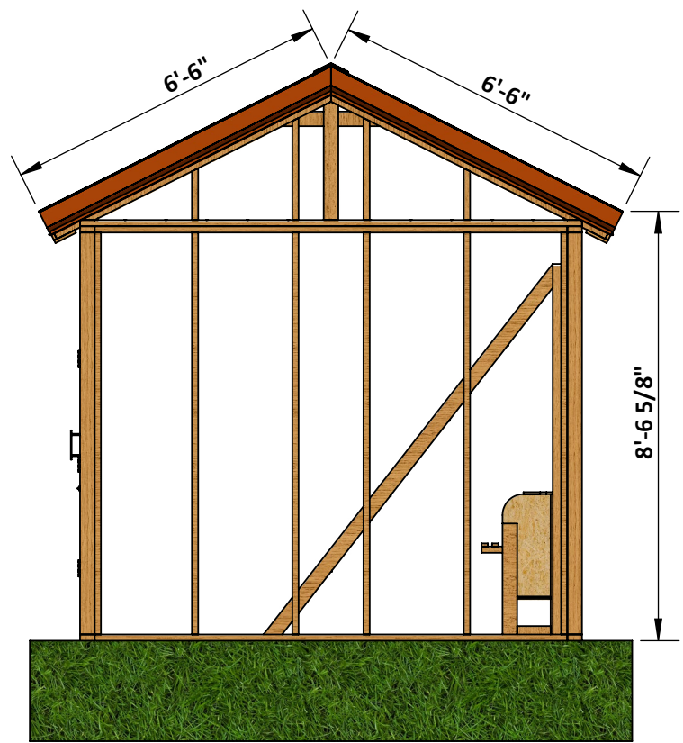
Roof Pitch 6/12
